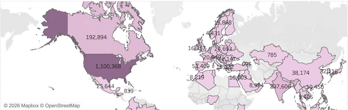
OS Distribution
